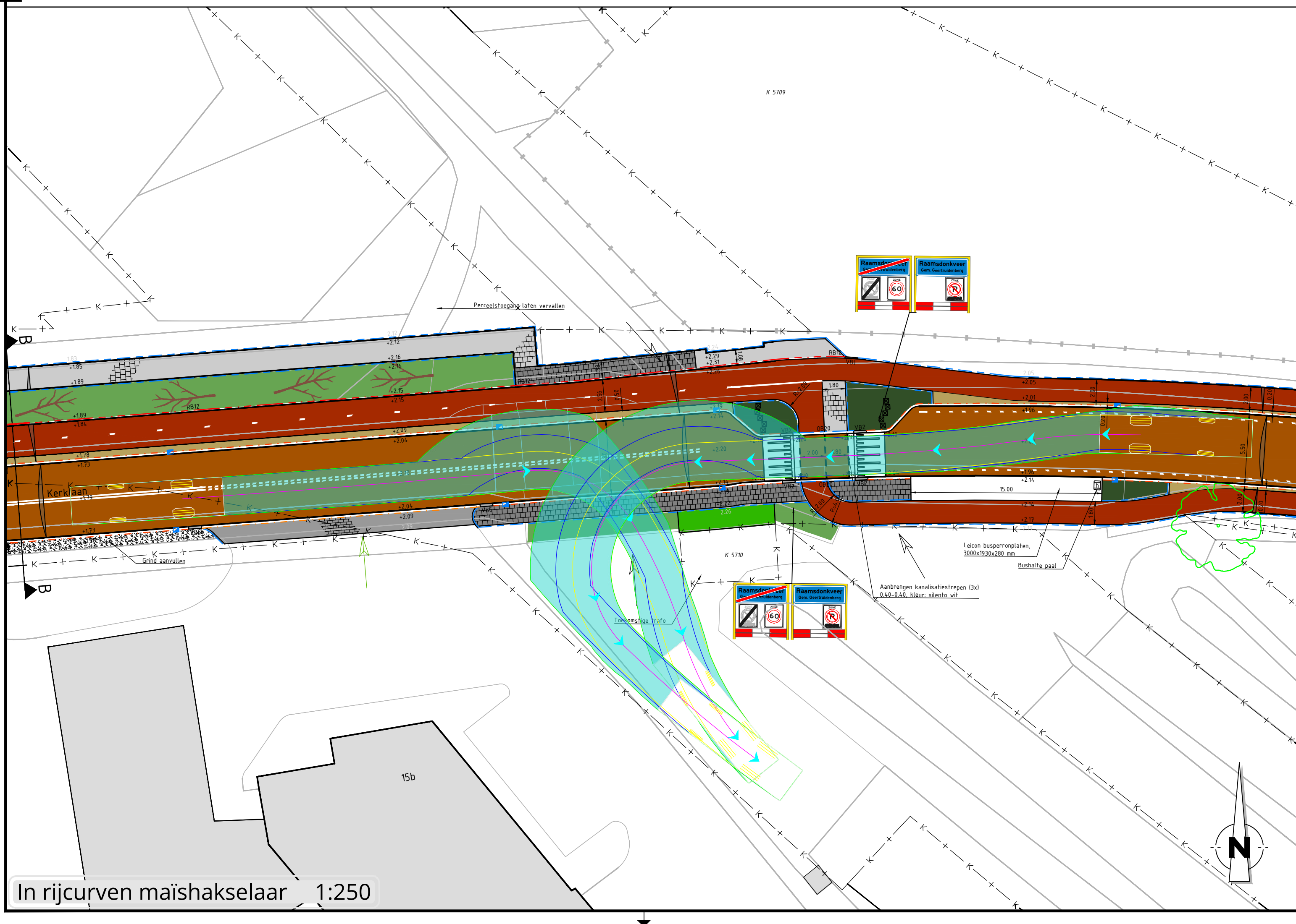
In rijcurven maishakselaar 1:250
